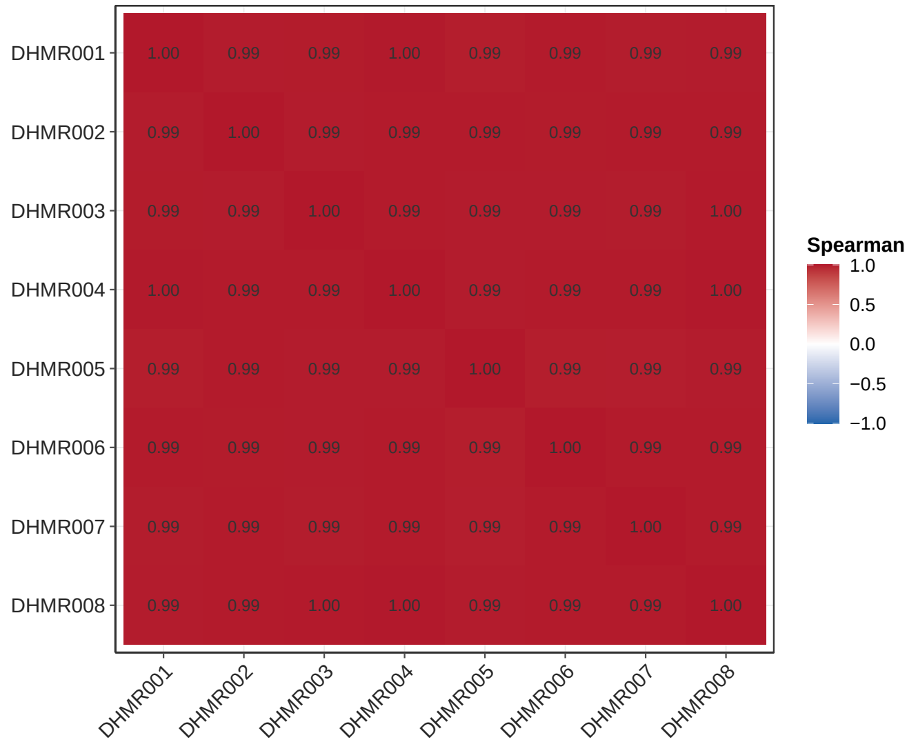
Sample-level correlation
